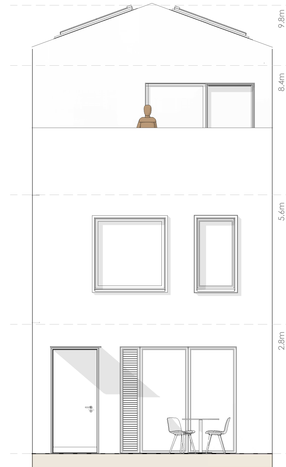
FRONT 1:50
