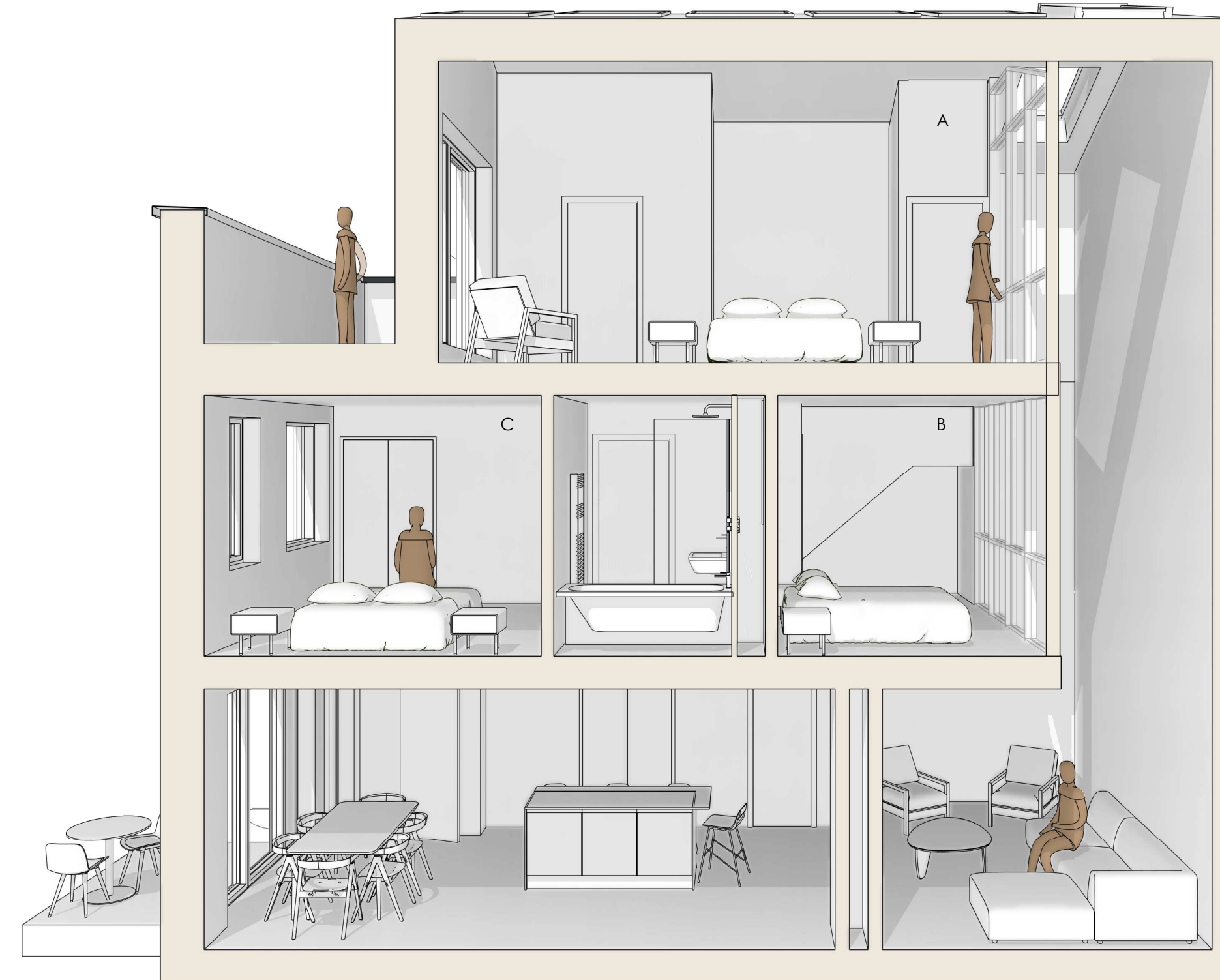
SECTION 1:50
